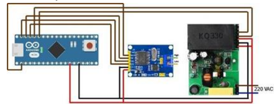
FIGURE 3.1 Wiring Diagram of EVPLC Module
