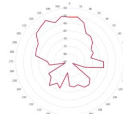
Figure 4.5 5 GHz Azimuth Radiation Pattern.
