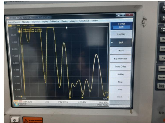
Figure 4.2 The results of the VSWR using VNA.
