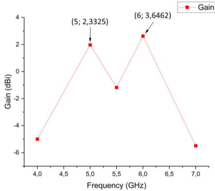
In Figure above, the gain for the 5 GHz is 2.3325 dBi while the gain for the 6 GHz is 3.6462 dBi.
