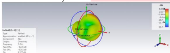
Figure 3.12 5 GHz radiation Pattern.
