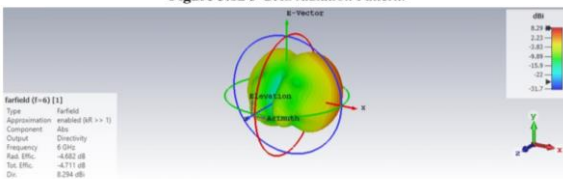
Figure 3.13 6 GHz radiation Pattern.
