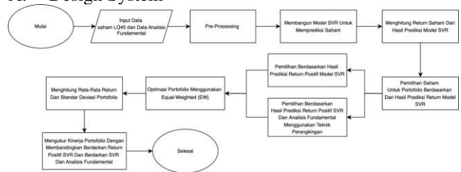
GAMBAR 1. Flowchart Design System
