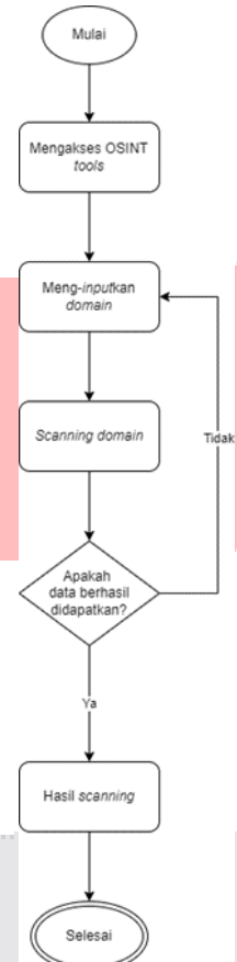
GAMBAR 2 Skenario Aktivitas Social Engineering
