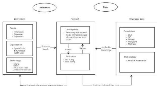
GAMBAR III.1 Model Konseptual
