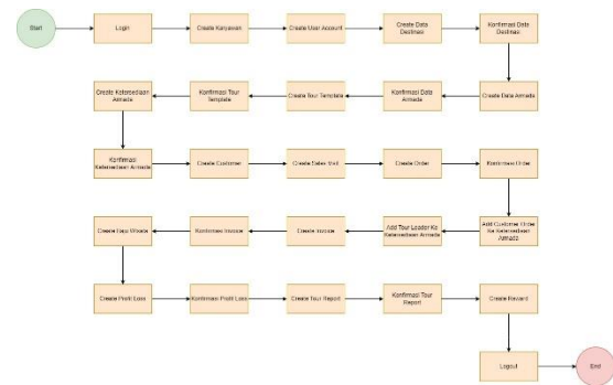
GAMBAR 4 User Flow
