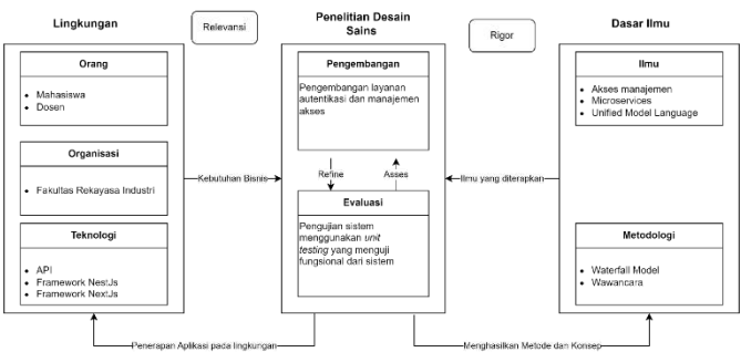
GAMBAR 3 Model Konseptual
