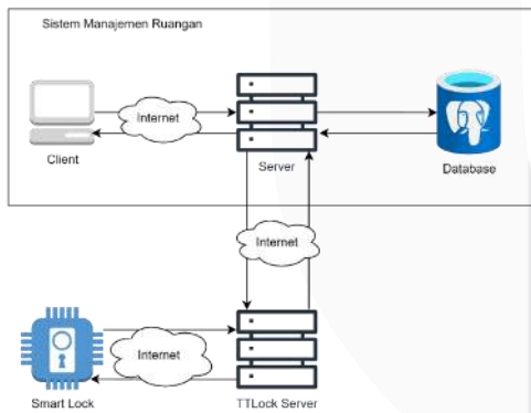
GAMBAR 5 Architecture diagram
