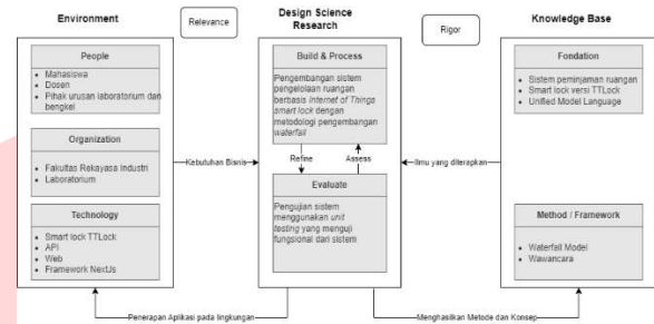
GAMBAR 2 Model Konseptual
