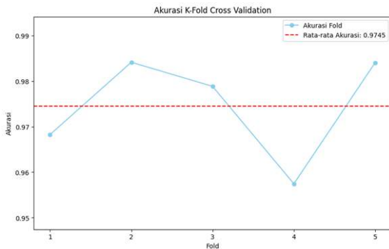
GAMBAR 8. K-Fold Cross Validation Sebelum Smote
