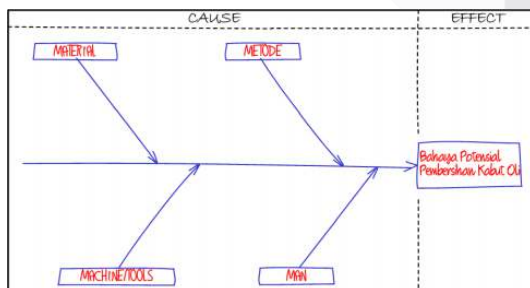
GAMBAR 4 Contoh Fishbone
