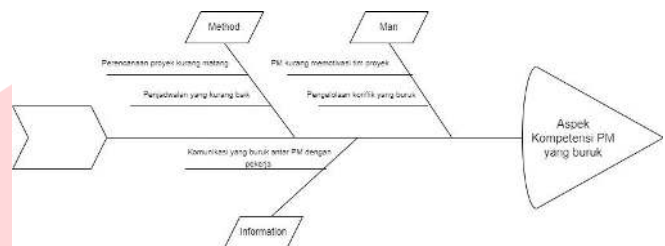
GAMBAR 2 Fishbone Diagram
