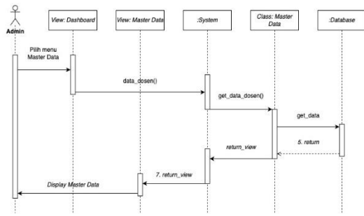
GAMBAR IV. 3 Sequence Diagram
