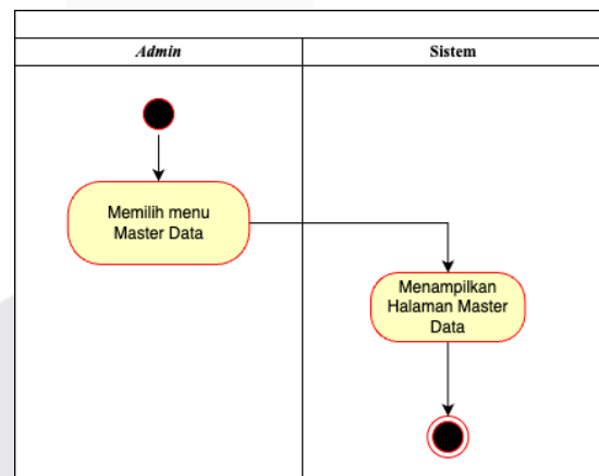
GAMBAR IV. 2 Activity Diagram
