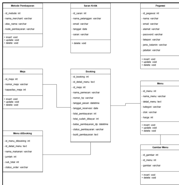
GAMBAR 18 (Class Diagram)
