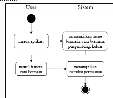
GAMBAR 4.5 (ACTIVITY DIAGRAM CARA BERMAIN)
