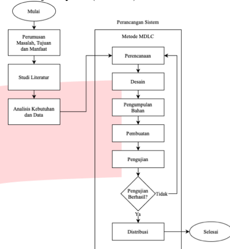
GAMBAR 3.1 (ALUR PENELITIAN)
