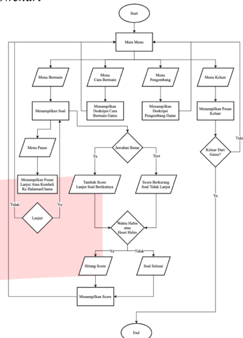
GAMBAR 4. 1 (FLOWCHART)
