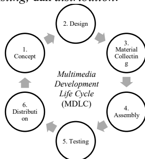
GAMBAR 2.1 (TAHAPAN MDLC)
