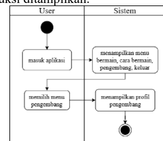
GAMBAR 4.6 ACTIVITY DIAGRAM PENGEMBANG
