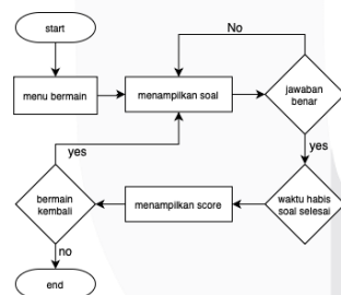
GAMBAR 4.2 (PLAY FLOW)
