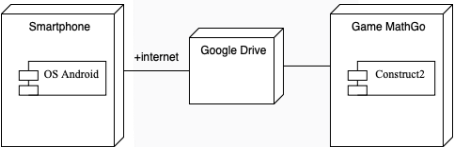
GAMBAR 4.8 (DEPLOYMENT DIAGRAM)
