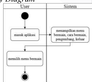
GAMBAR 4.3 (ACTIVITY DIAGRAM MAIN MENU)
