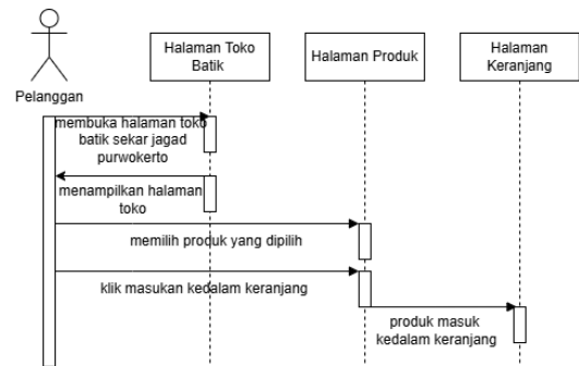
GAMBAR 4.4 (SEQUENCE DIAGRAM)
