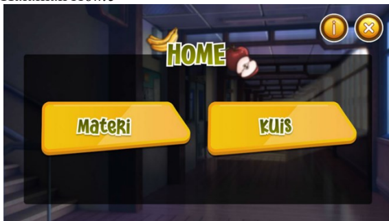
GAMBAR 3 (HALAMAN HOME )
