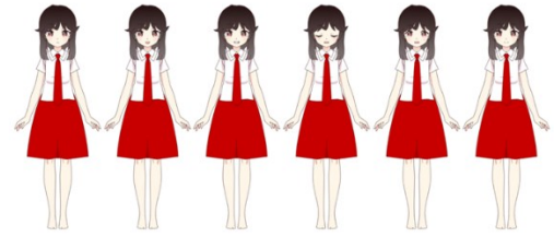
GAMBAR 10 (CHAR EVA)
