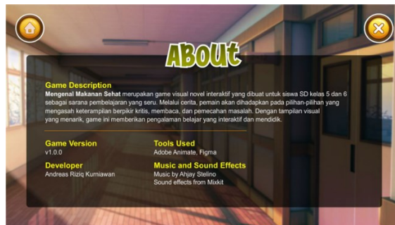
GAMBAR 6 (HALAMAN ABOUT )
