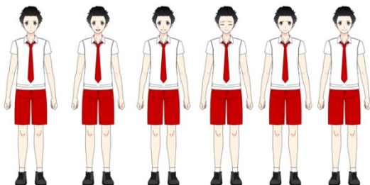
GAMBAR 9 (CHAR BOY)
