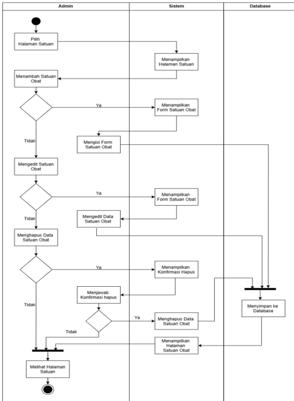
GAMBAR 8 (Activity Diagram Halaman Satuan Obat)
