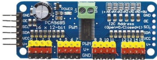
GAMBAR 8 (DRIVER SERVO MOTOR PCA9685 [15])
