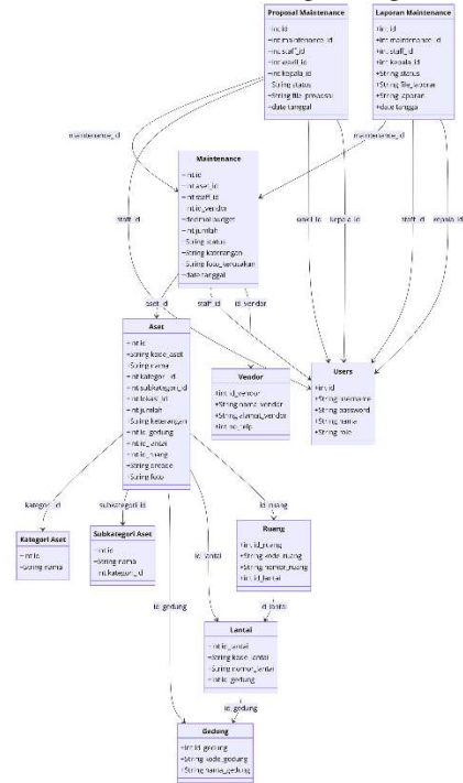
FIGURE IV. 4 Class Diagram
