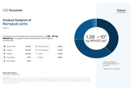
GAMBAR 1.5 PHOTOCHEMICAL OXIDATION
