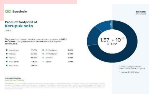
GAMBAR 1. 4 HUMAN TOXICITY
