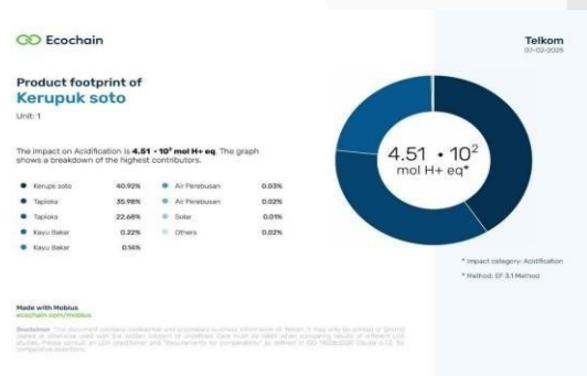
GAMBAR 1. 3 ACIDIFICATION
