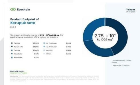
GAMBAR 1. 1 CLIMATE CHANGE
