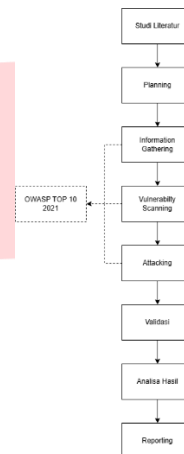
GAMBAR 1 (ALUR PENELITIAN)
