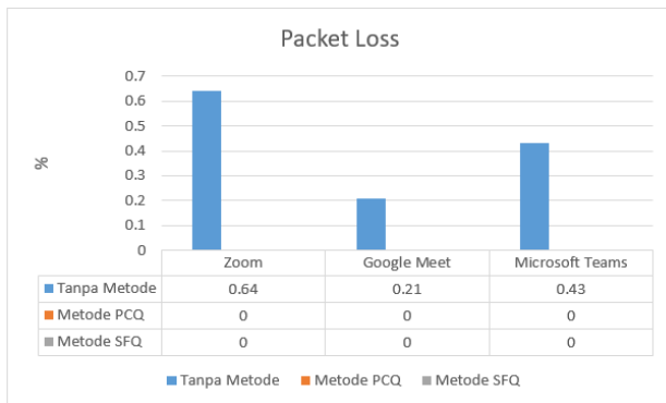
GAMBAR 6 (PACKET LOSS)
