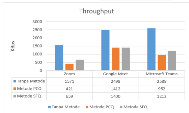
GAMBAR 7 (THROUGHPUT)
