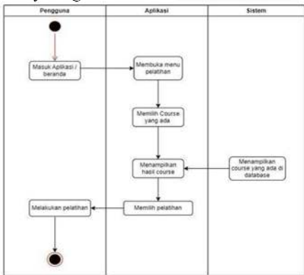
GAMBAR 3.2 Activity Diagram
