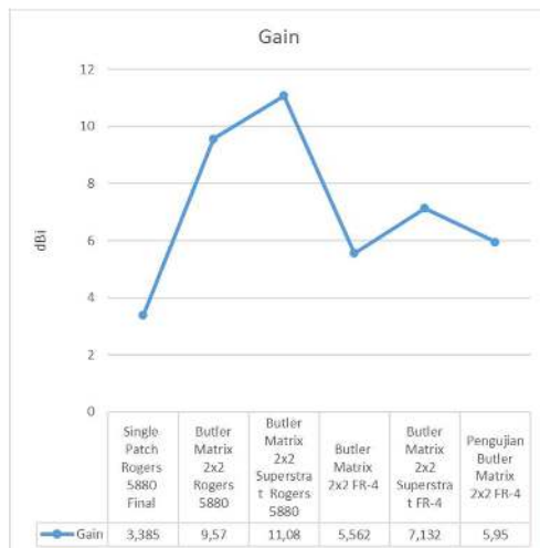
GAMBAR 9 Perbandingan Hasil Gain.
