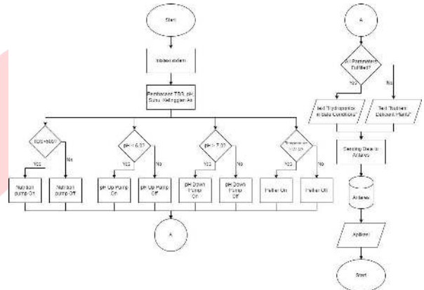
GAMBAR 6 Flowchart AWNDES
