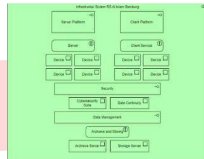
GAMBAR 15 Platform Decomposition Diagram
