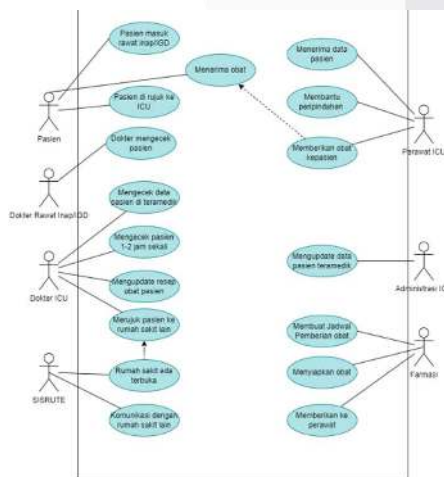
GAMBAR 13 Use Case Diagram
