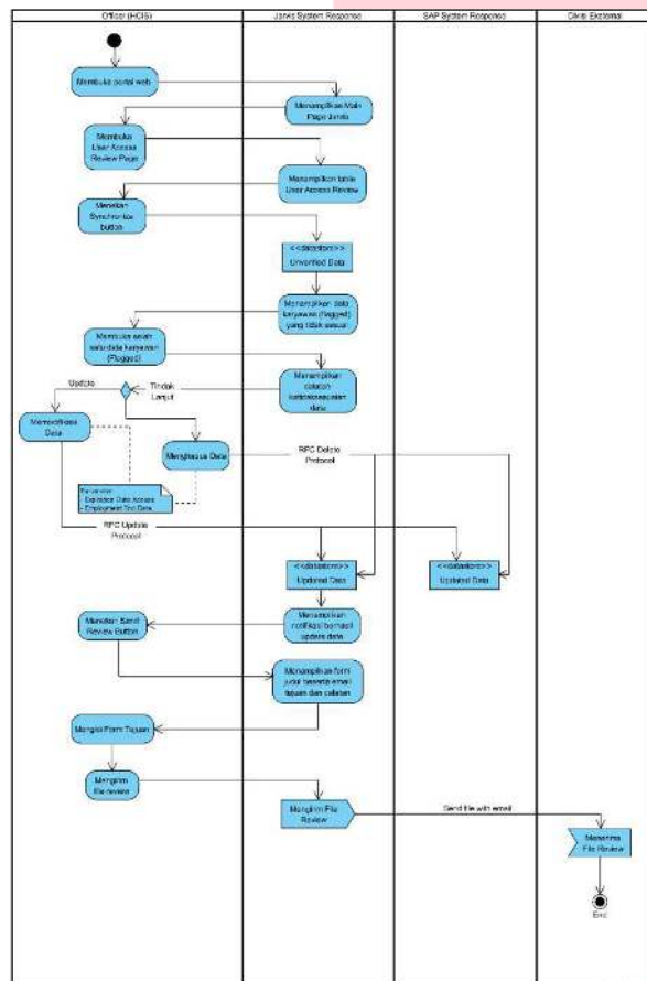
GAMBAR 7 (Activity Diagram User Access Review)
