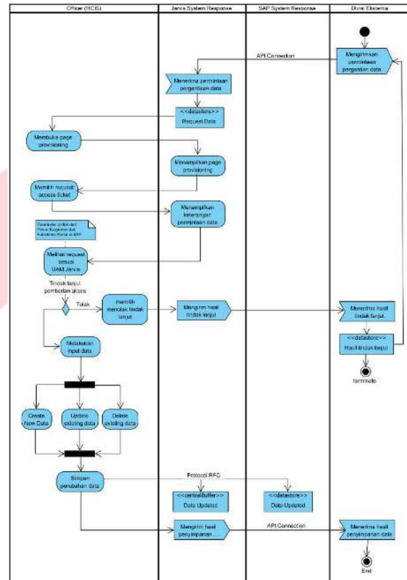
GAMBAR 8 (Activity Diagram Provisioning)
