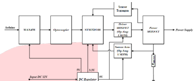
GAMBAR 3 (BLOK DIAGRAM MODULE DC ELECTRONIC LOAD)
