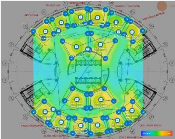
GAMBAR 5 Heatmap Signal Level Lantai 10
