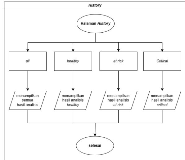
GAMBAR 7 Flowchart Sub-proses Halaman History
