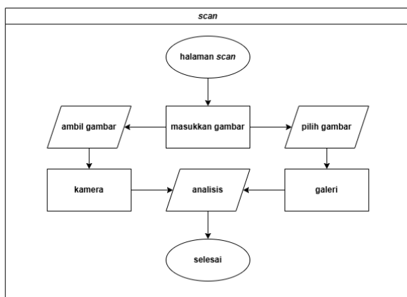
GAMBAR 6 Flowchart Sub-proses Halaman Scan
