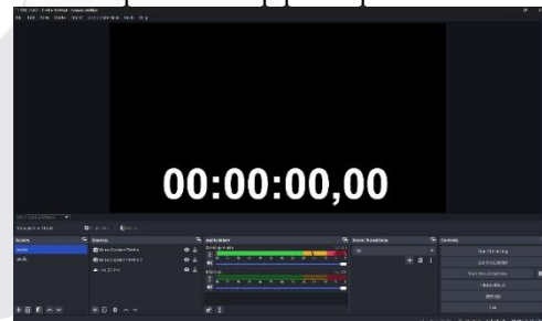
GAMBAR 20 (OBS Studio)
