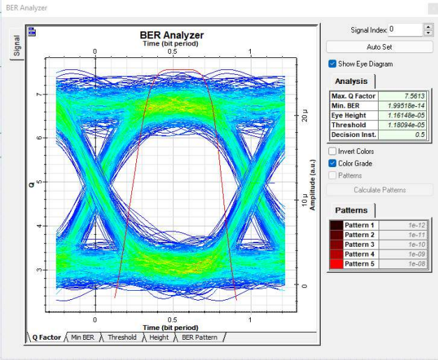
GAMBAR 13 HASIL SIMULASI Q-FACTOR
