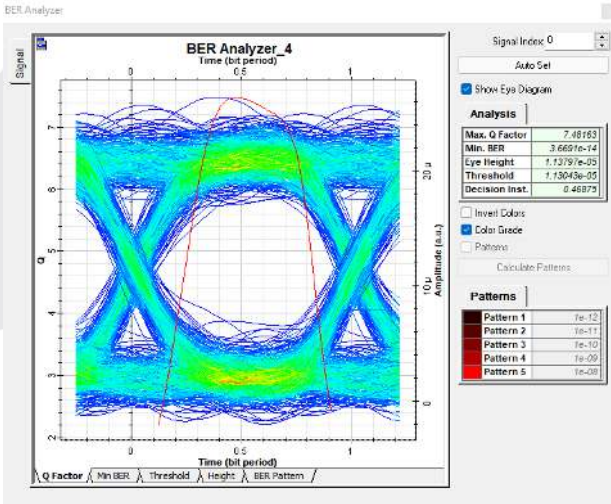
GAMBAR 14 HASIL SIMULASI Q-FACTOR
