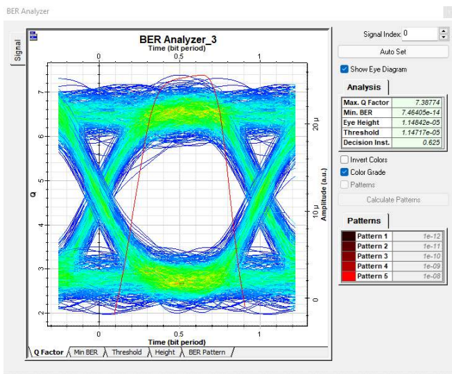
Gambar 4. 1 Hasil simulasi Q-factor
