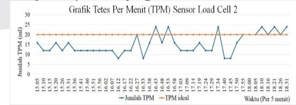
GAMBAR 9 GRAFIK TPM SENSOR LOADCELL 2
