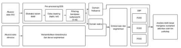
GAMBAR 3 (Flowchart Sistem)
