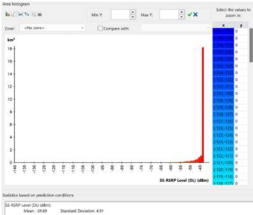
GAMBAR 4 Histogram SS-RSRP
