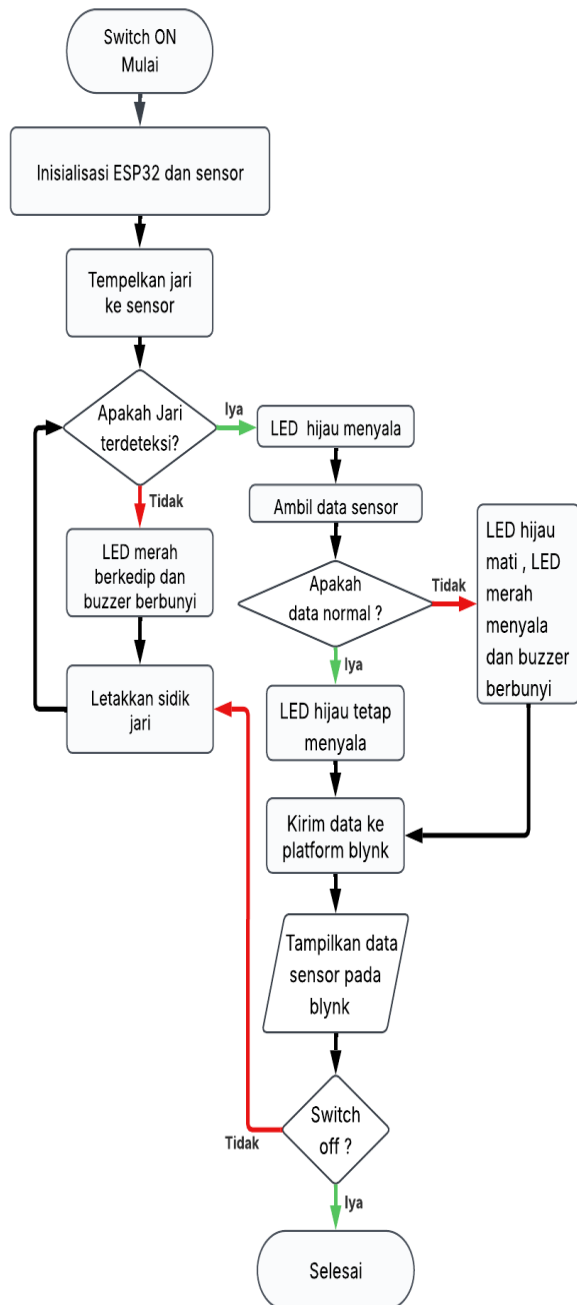
GAMBAR 2. FLOWCHART SISTEM ESP32
