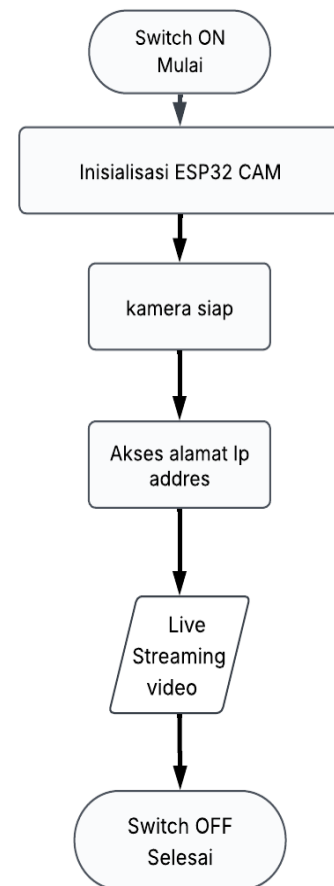
GAMBAR 3. FLOWCHART SISTEM ESP32-CAM
