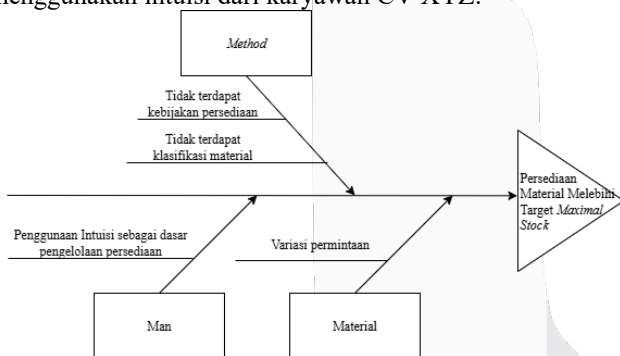
GAMBAR 2 Fishbone Diagram
