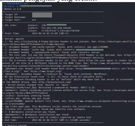
GAMBAR 3 HASIL SCANNING NIKTO
