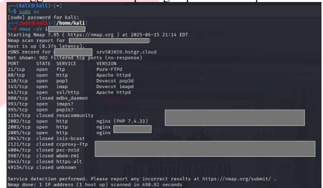
GAMBAR 4 HASIL SCANNING NMAP
