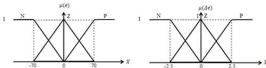
Gambar 10. Membership function 3
