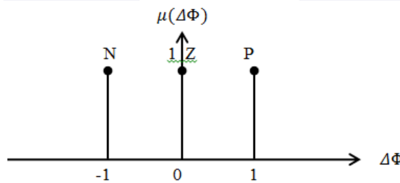
Gambar 9. Output 2
