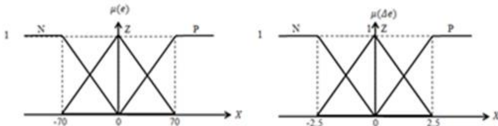
Gambar 7. Membership function 1
