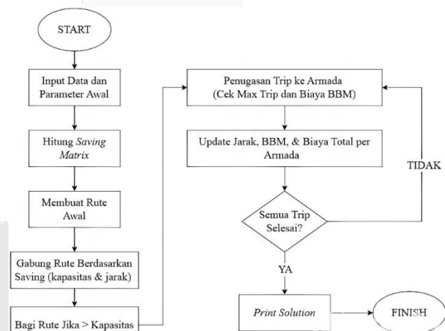
GAMBAR 9 Flowchart Diagram
