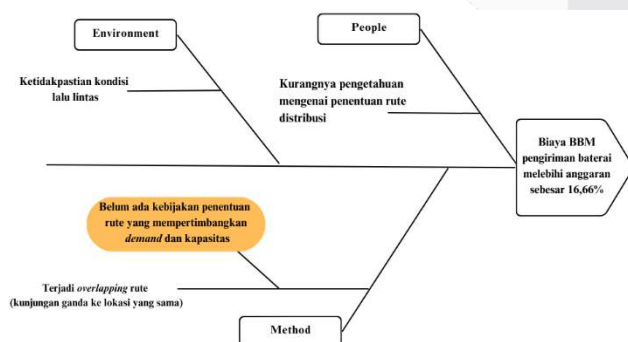
GAMBAR 4 Fishbone Diagram
