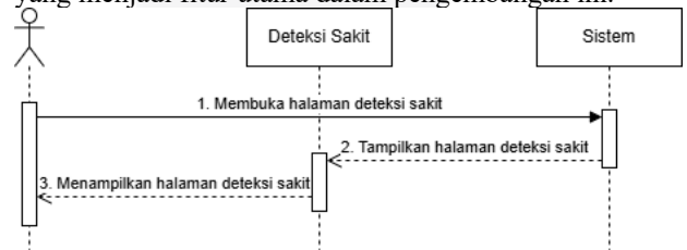
GAMBAR 5 SEQUENCE DIAGRAM DETEKSI SAKIT
