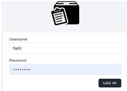
GAMBAR 2 (LOGIN PAGE)
