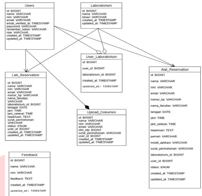
GAMBAR 4 (CLASS DIAGRAM)
