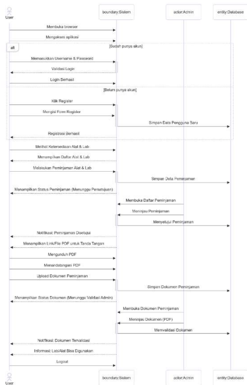
GAMBAR 6 (SEQUENCE DIAGRAM)
