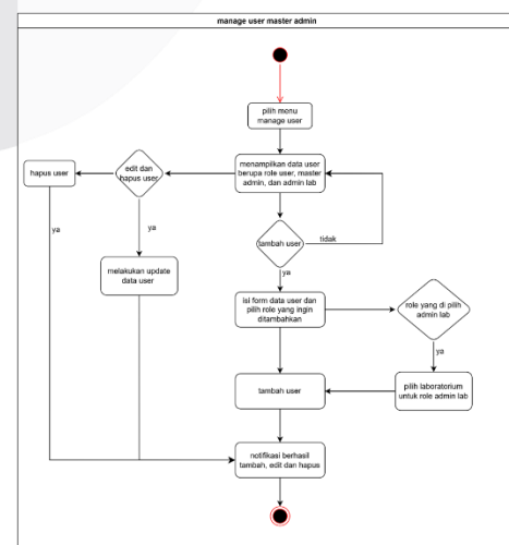
GAMBAR 5 (ACTIVITY DIAGRAM)
