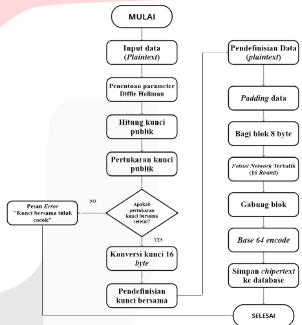
GAMBAR 10 (PENGINTEGRASIAN MODEL DEKRIPSI)
