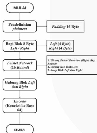
GAMBAR 8 (MODEL ENKRIPSI BLOWFISH)
