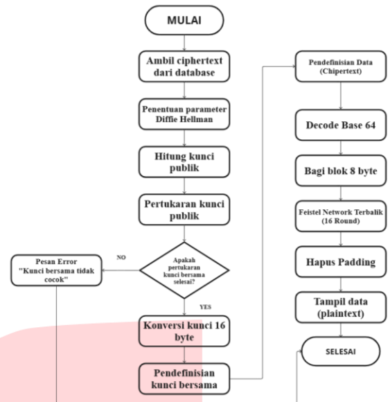
GAMBAR 9 (PENGINTEGRASIAN MODEL ENKRIPSI)
