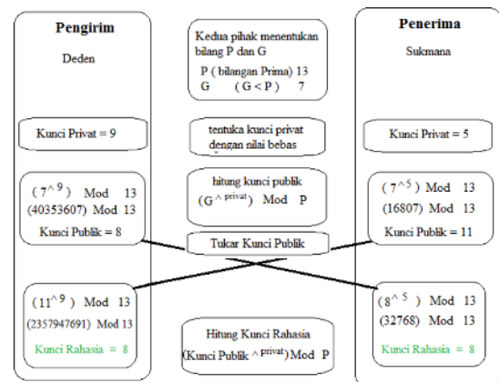
GAMBAR 3 (ILUSTRASI PERTUKARAN KUNCI DIFFIE HELLMAN)
