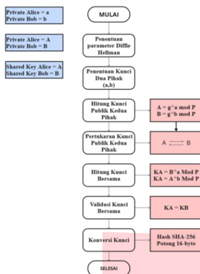
GAMBAR 7 (PROSES PERTUKARAN KUNCI DIFFIE HELMAN)
