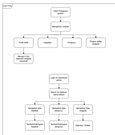
GAMBAR 4 (USER FLOW DIAGRAM)
