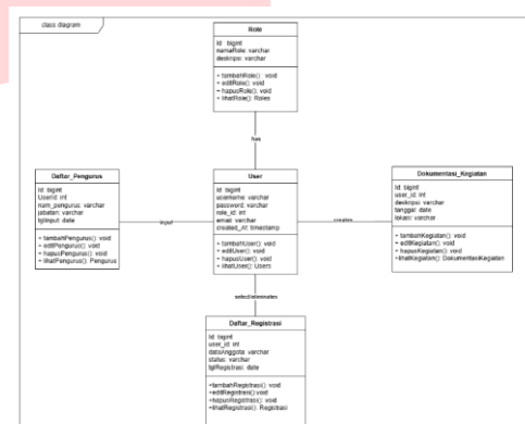
GAMBAR 7 (CLASS DIAGRAM)
