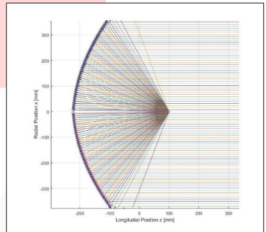
Gambar 7 Ray Tracing
