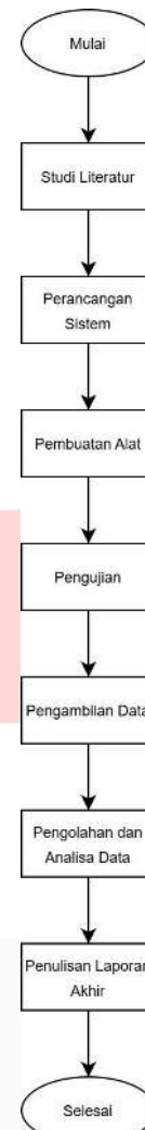
GAMBAR 1 (ALUR PENELITIAN)
