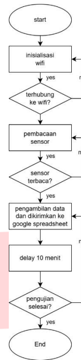
GAMBAR 4 (ALUR PROGRAM)
