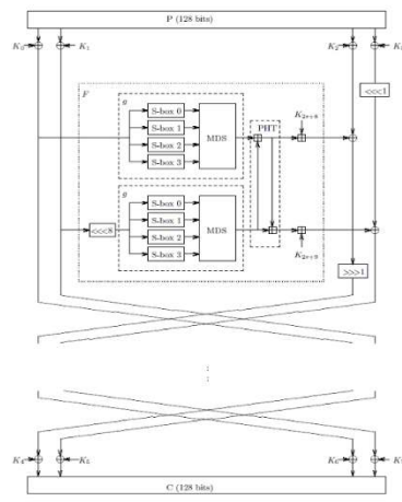
GAMBAR 1 (BLOK DIAGRAM TWOFISH)
