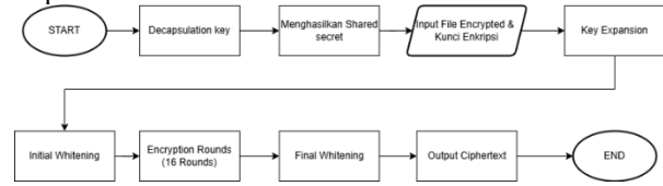
GAMBAR 6 (DEKRIPSI TWOFISH)
