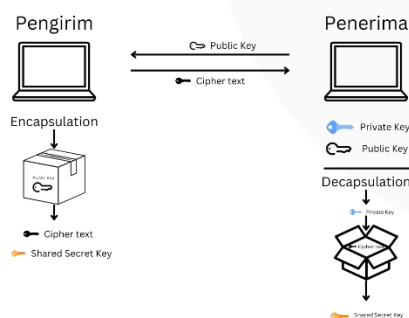
GAMBAR 2 (ENCAPSULATION MECHANISM)
