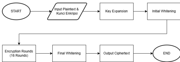
GAMBAR 5 (ENKRIPSI TWOFISH)
