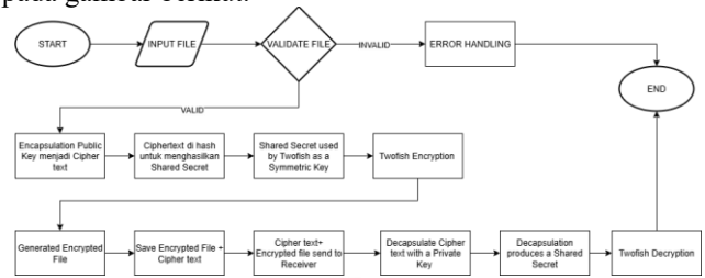
GAMBAR 3 (ALUR PENELITIAN)
