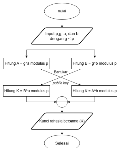
GAMBAR 6 (ALUR DIFFIE-HELLMAN)
