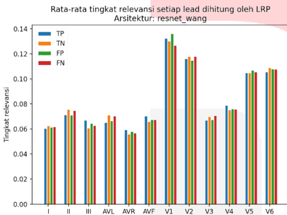
GAMBAR 10 Lead relevance score ResNet
