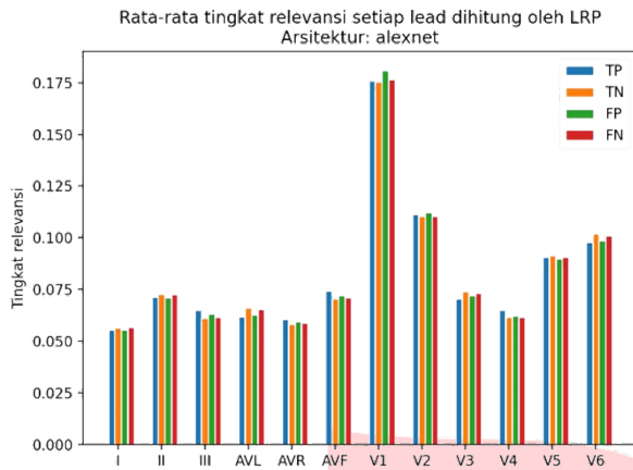
GAMBAR 9 Lead relevance score AlexNet 1D
