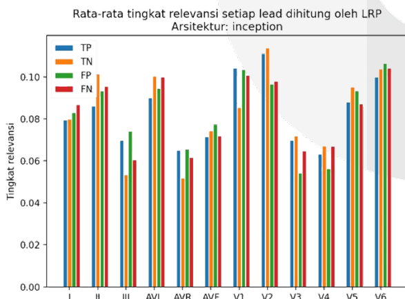
GAMBAR 11 Lead relevance score Inception
